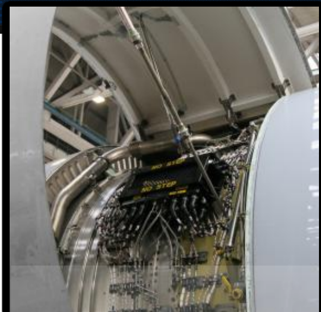
Engine Brackets
